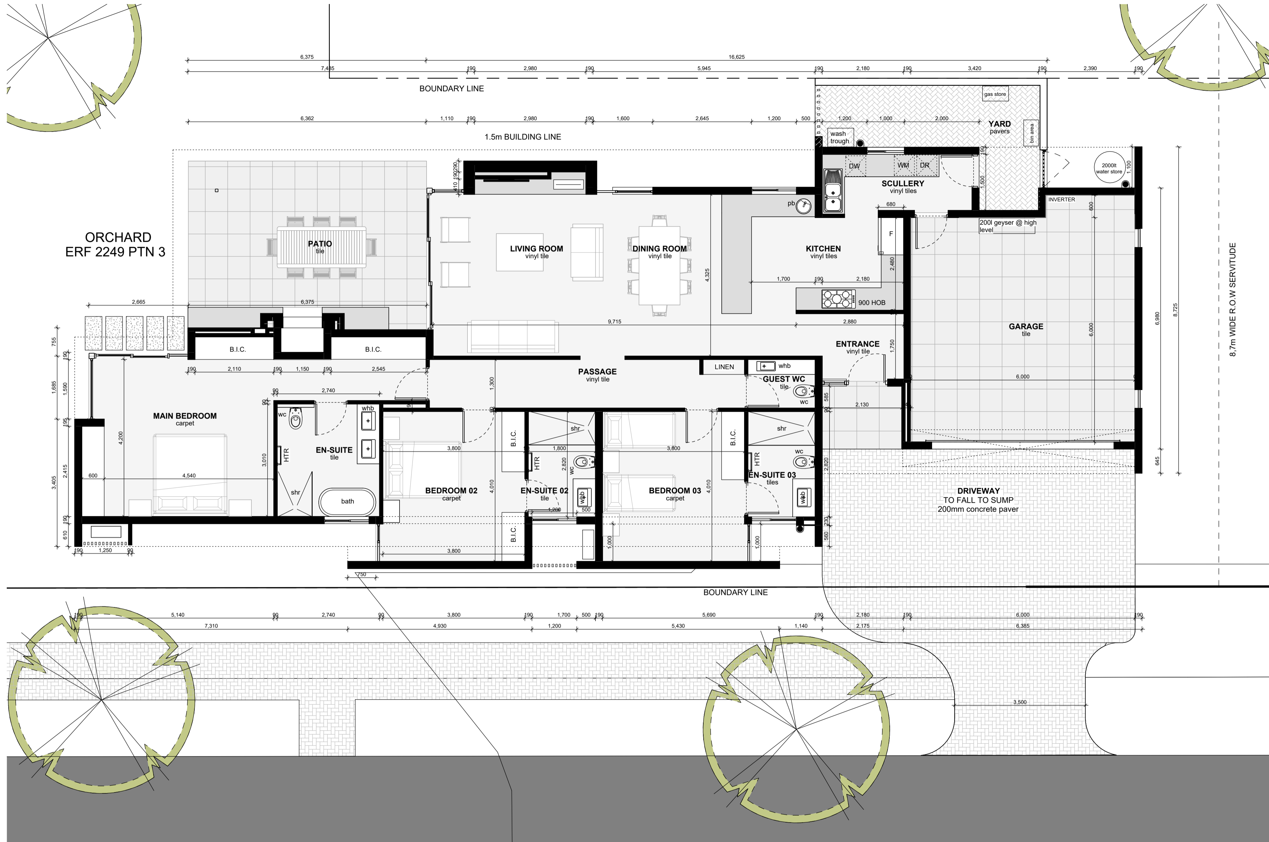
1 Ground Floor Plan - Marketing plan 1 : 50
