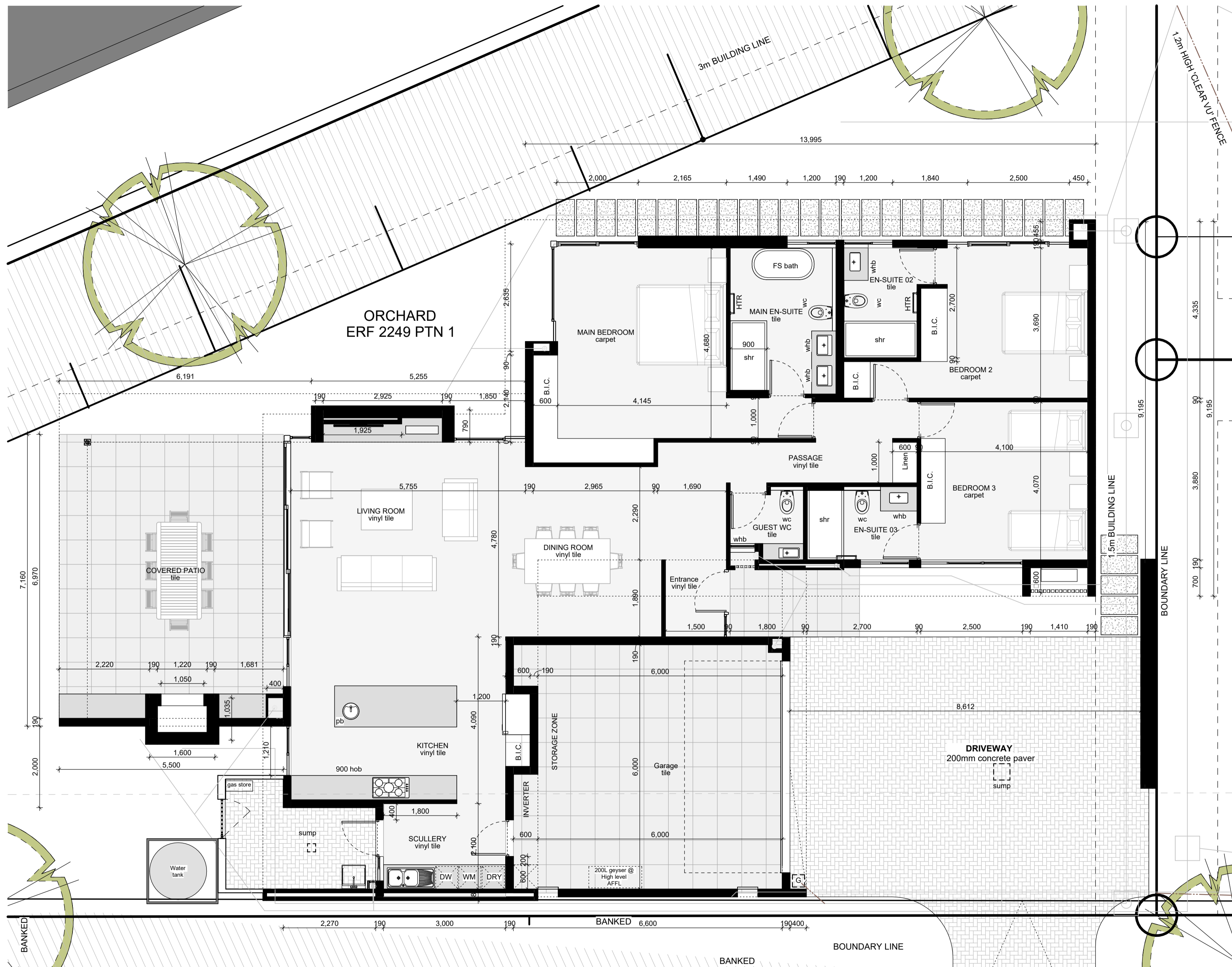
1 Ground Floor - Marketing plan 1 : 50
