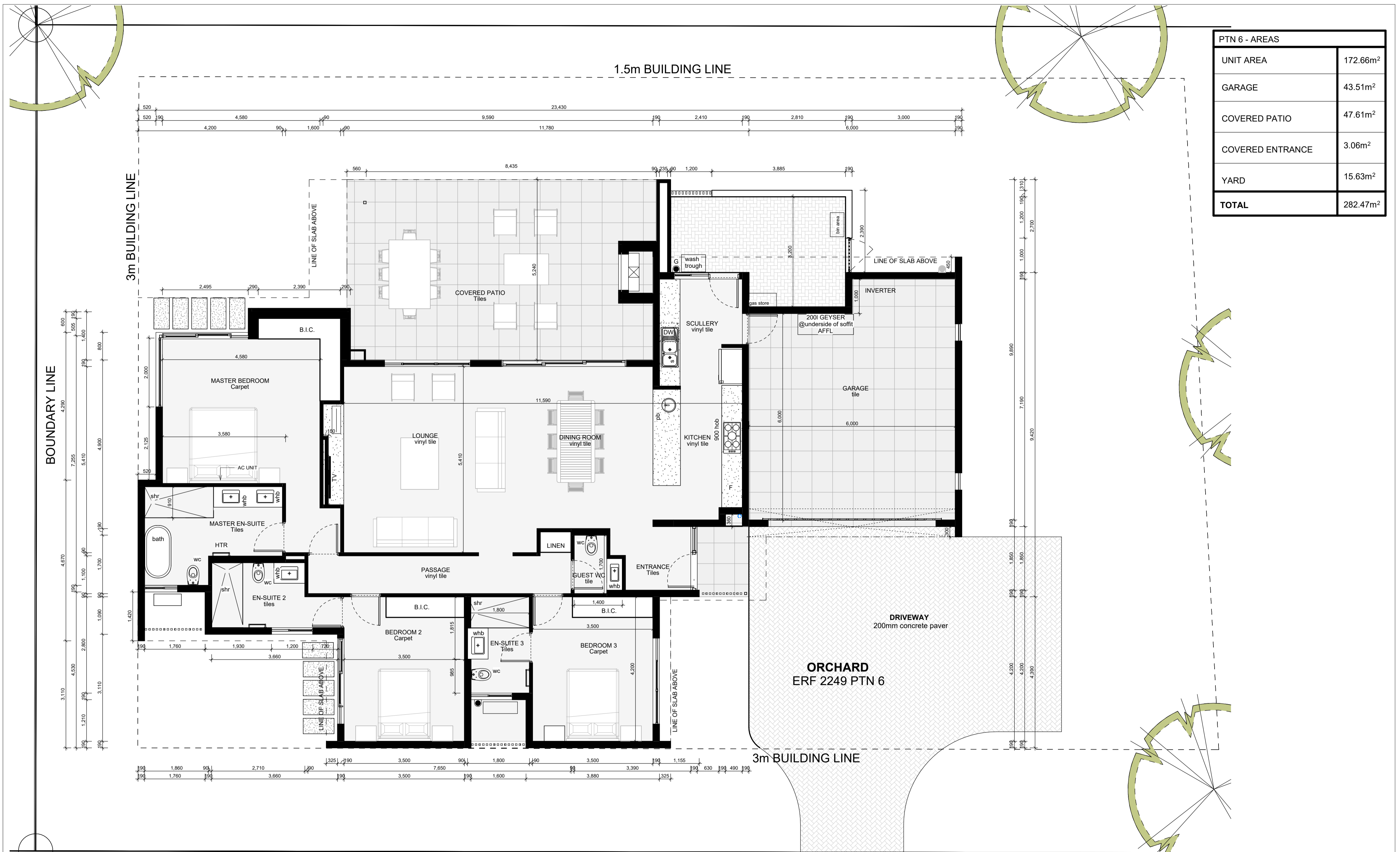
1 Ground Floor Plan - Marketing plan 1 : 50
